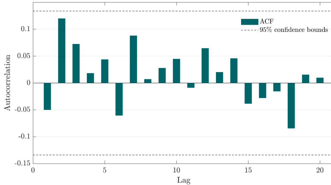
Figure C.1. Autocorrelation test
